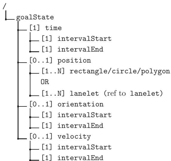
Figure 11: Element goal state of a planning problem
