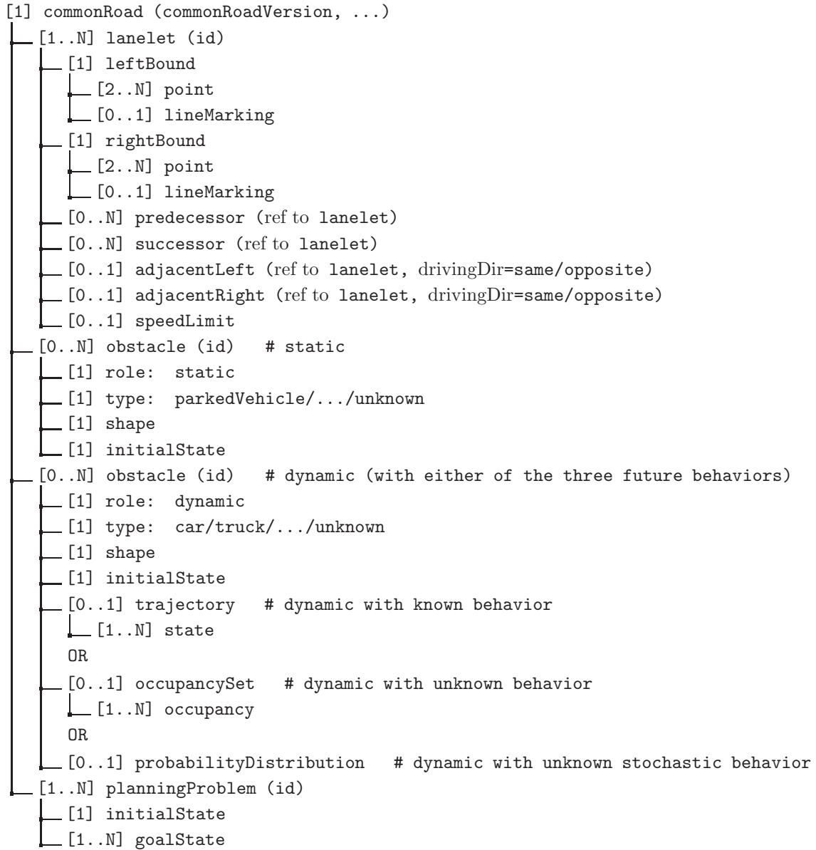
Figure 1: Structure of the XML files encoding each scenario
